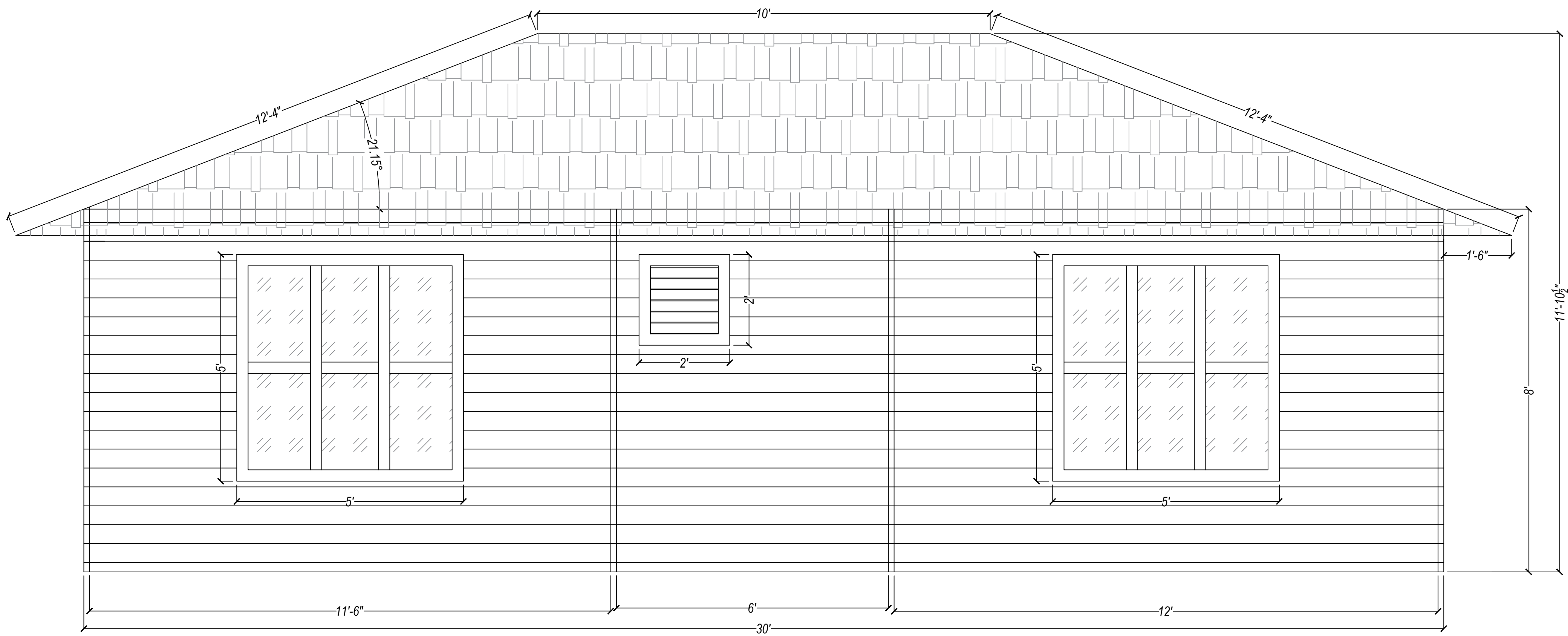
Back Elevation
