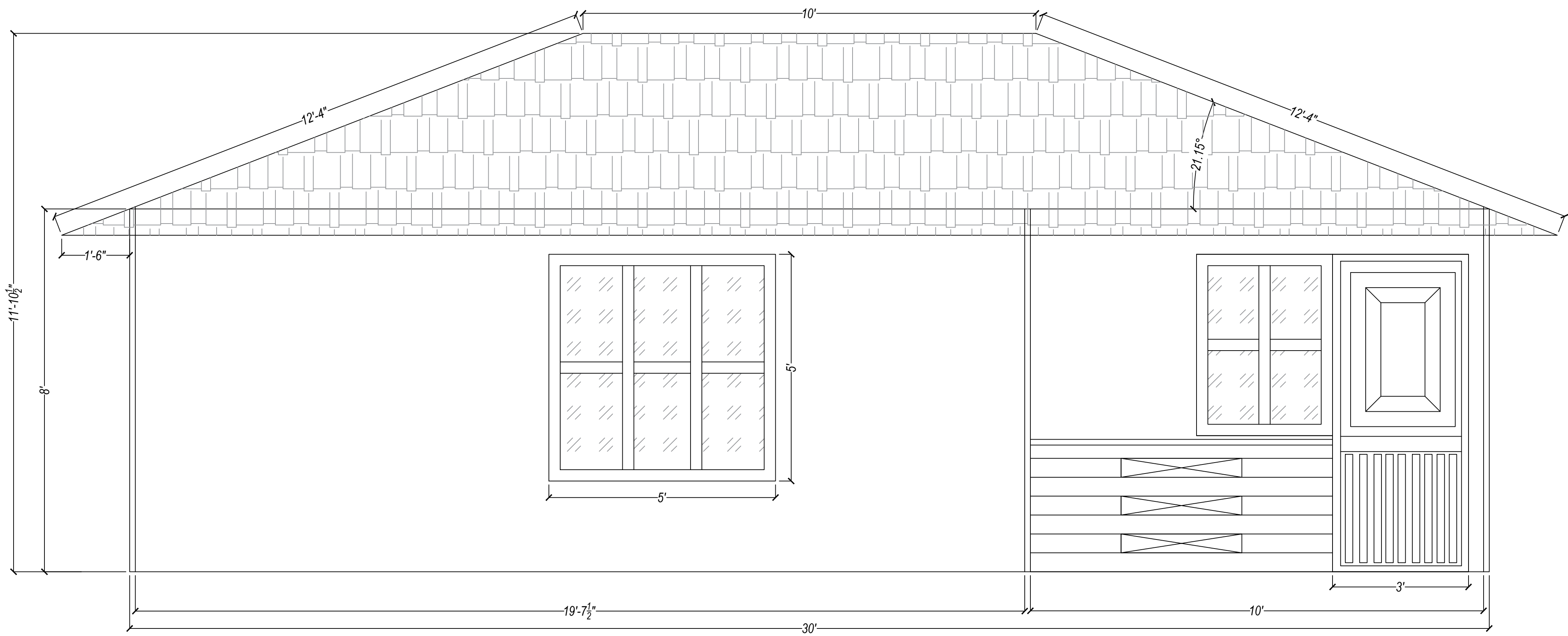
Front Elevation with Balcony
