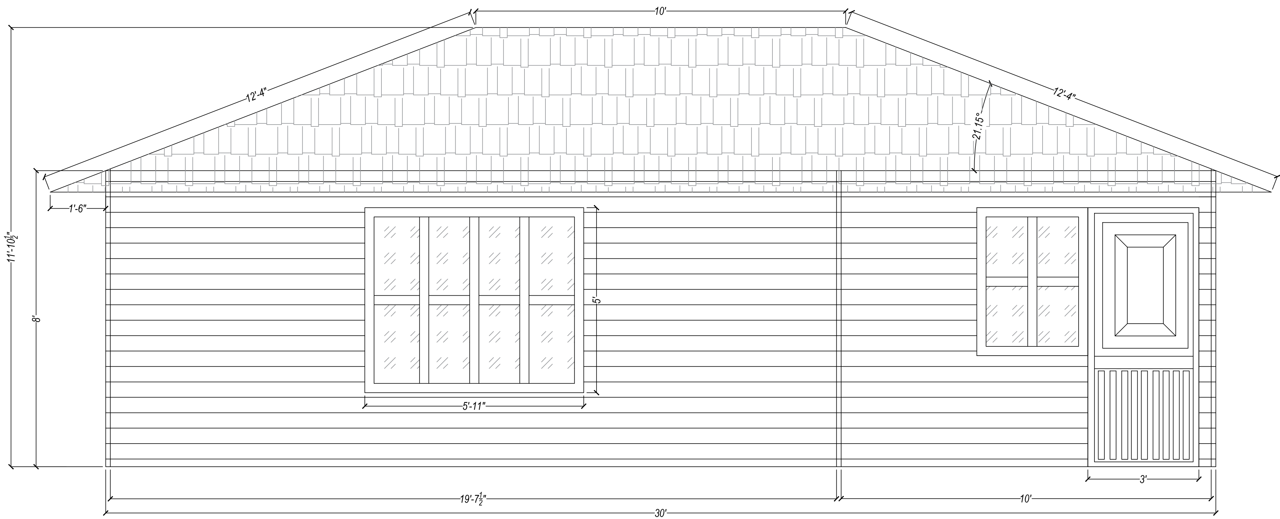
Front Elevation
