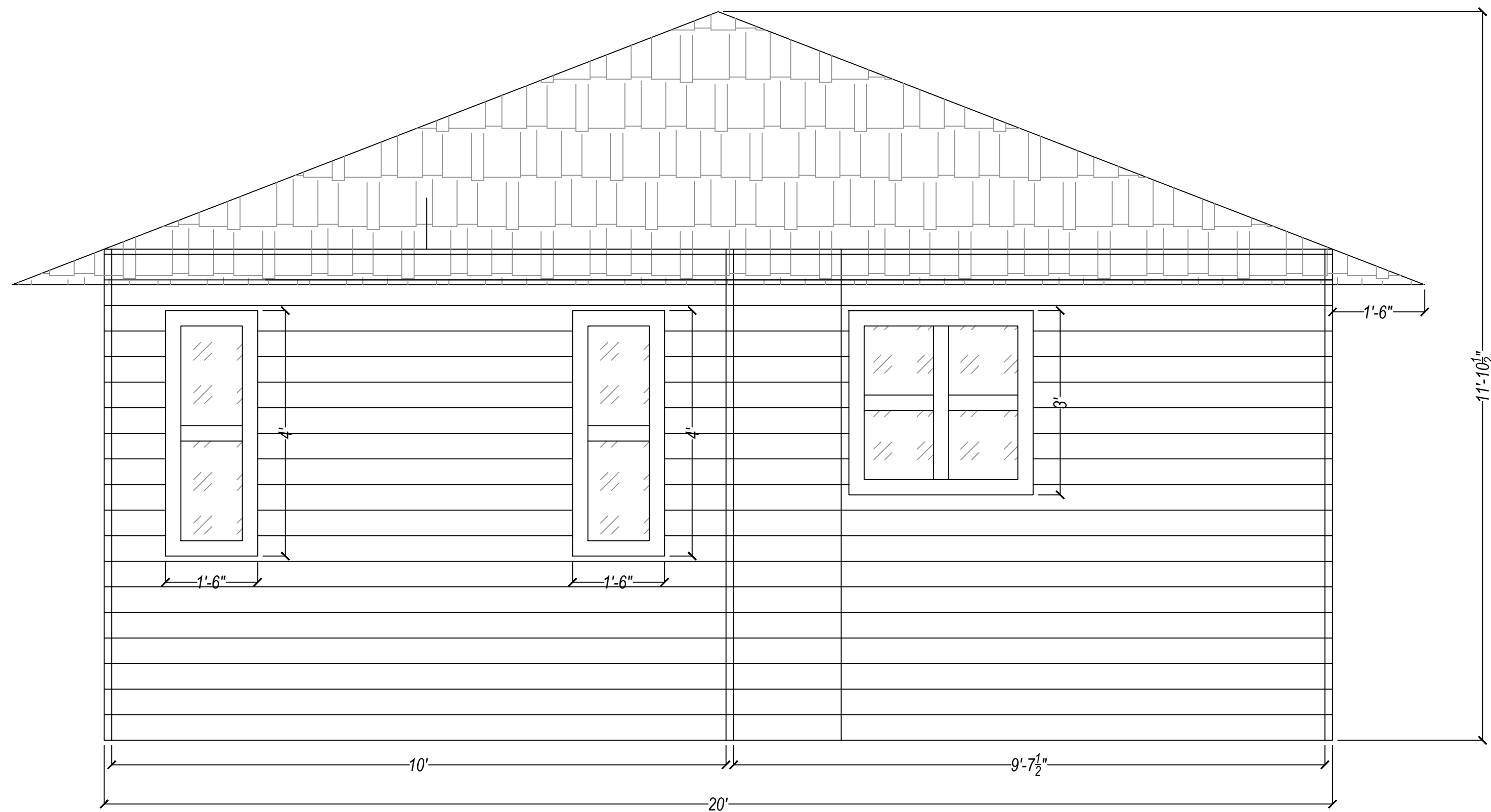
Left Elevation
