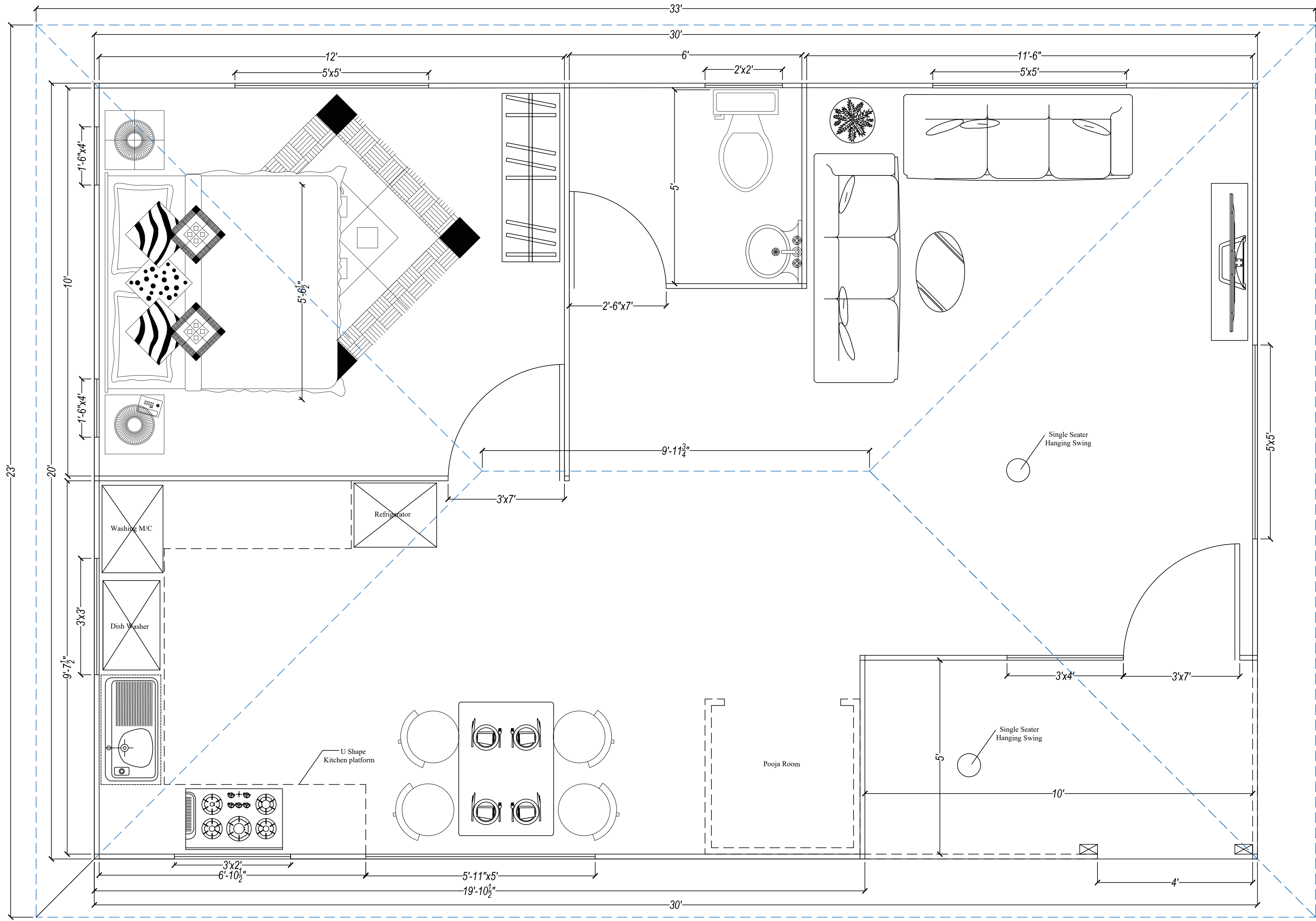
Floor Plan
