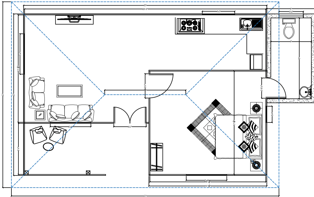
Floor Plan
