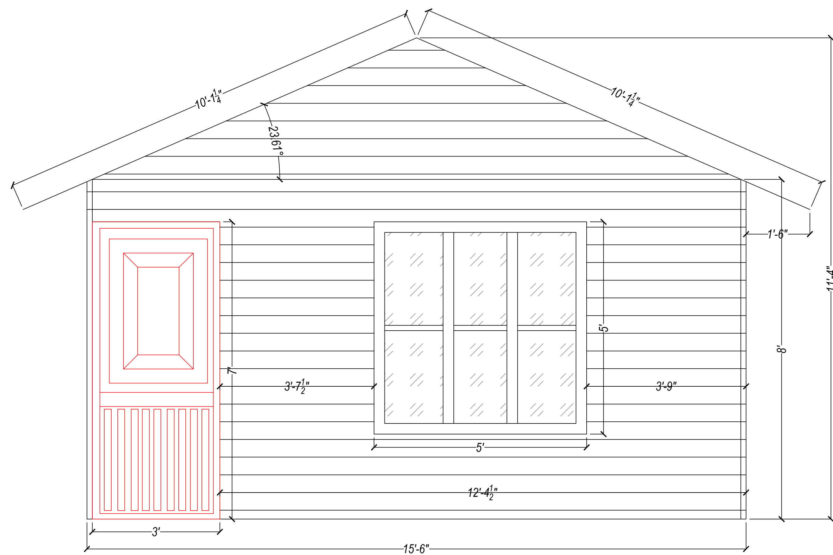
Front Elevation
