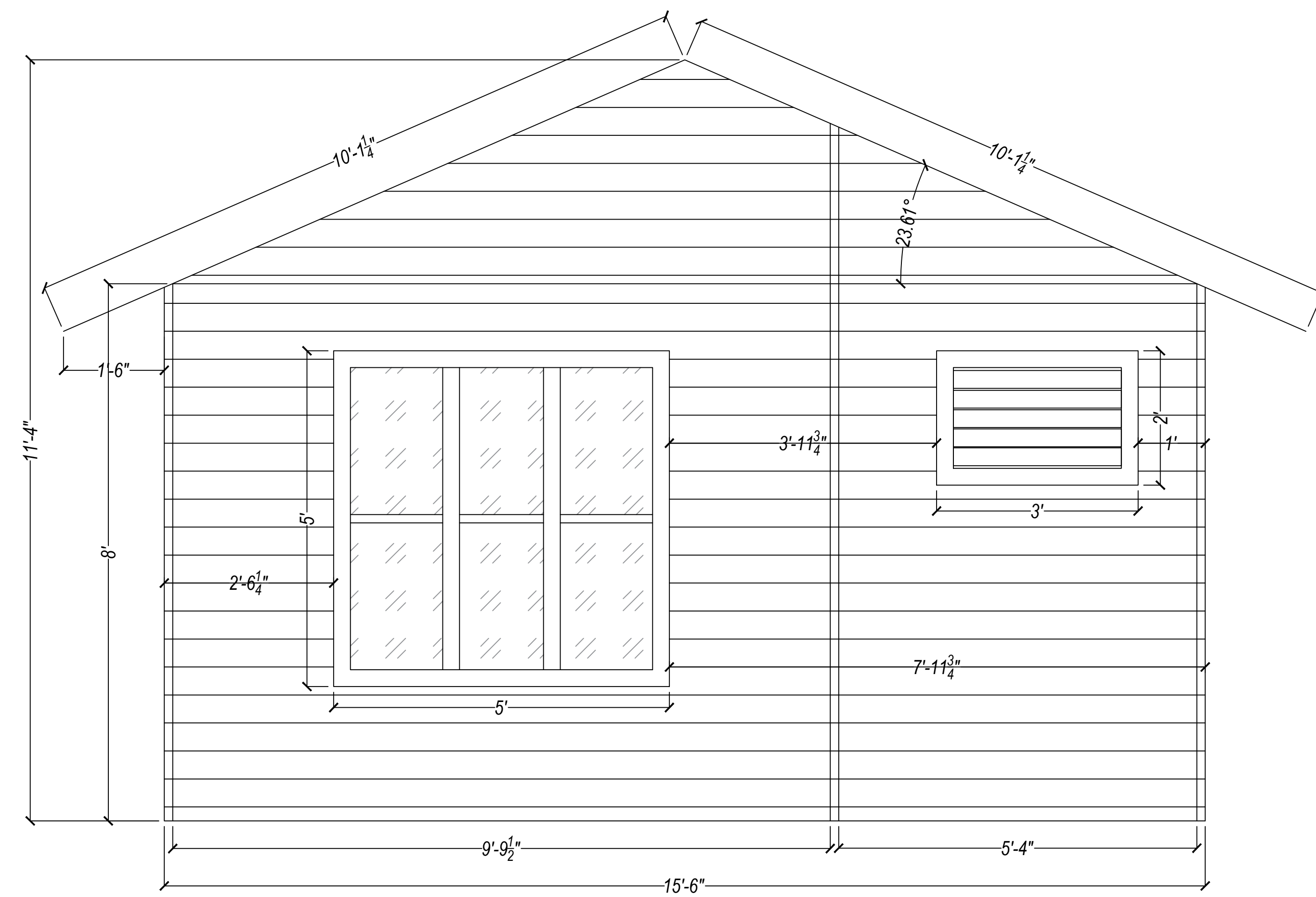
Back Elevation
