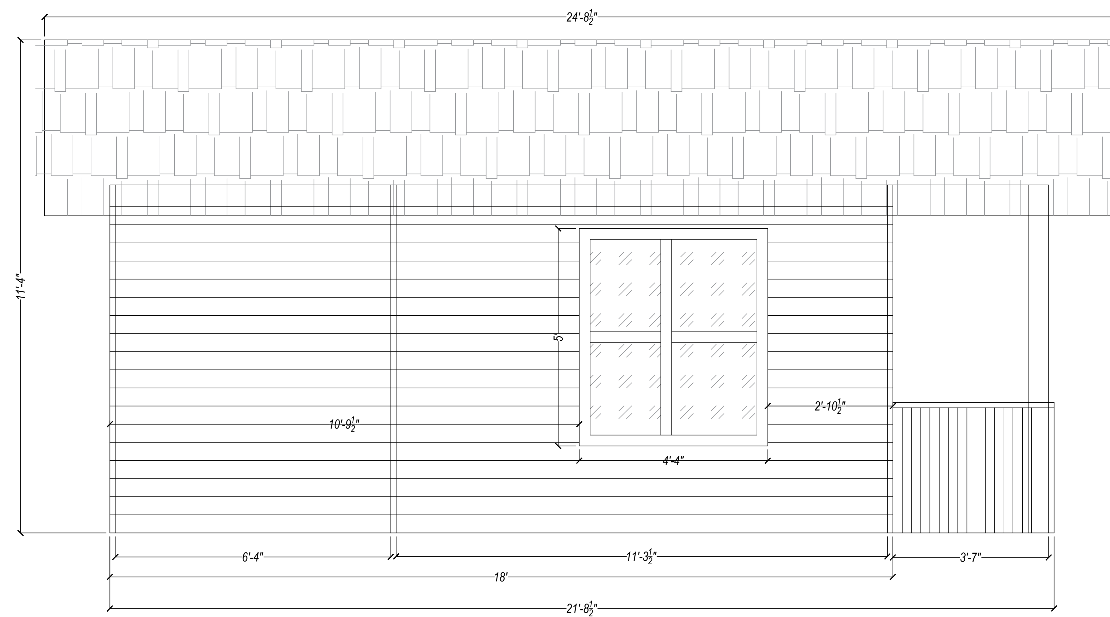
Left Elevation
