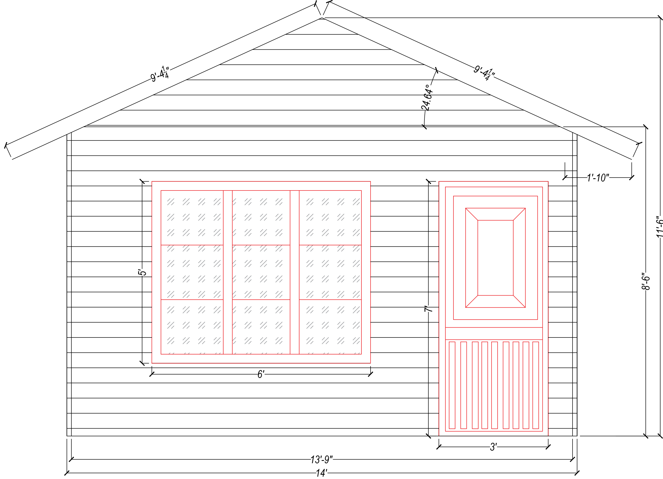
Front Elevation
