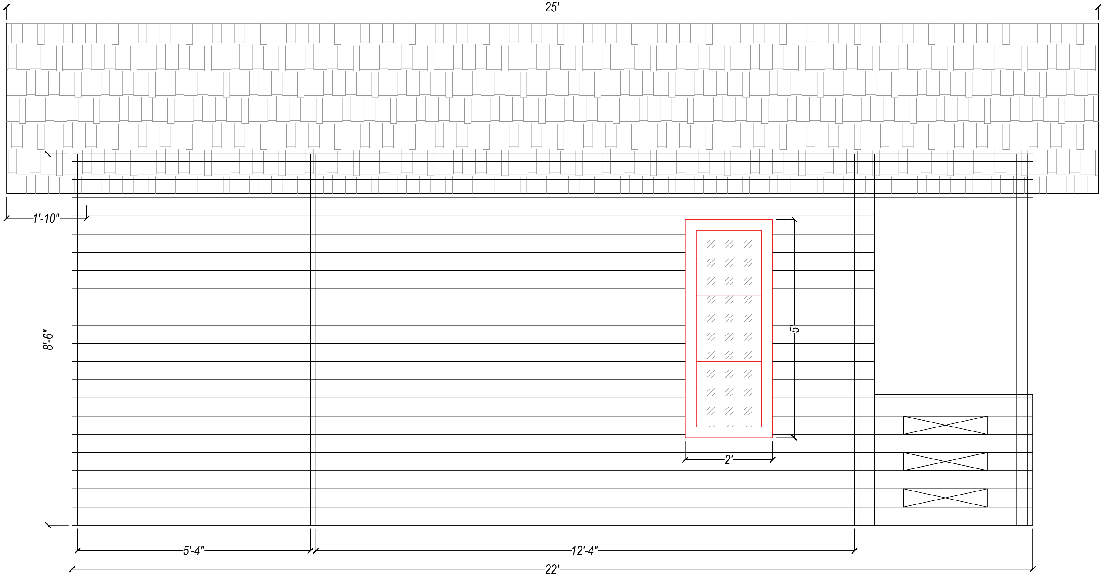
Left Elevation
