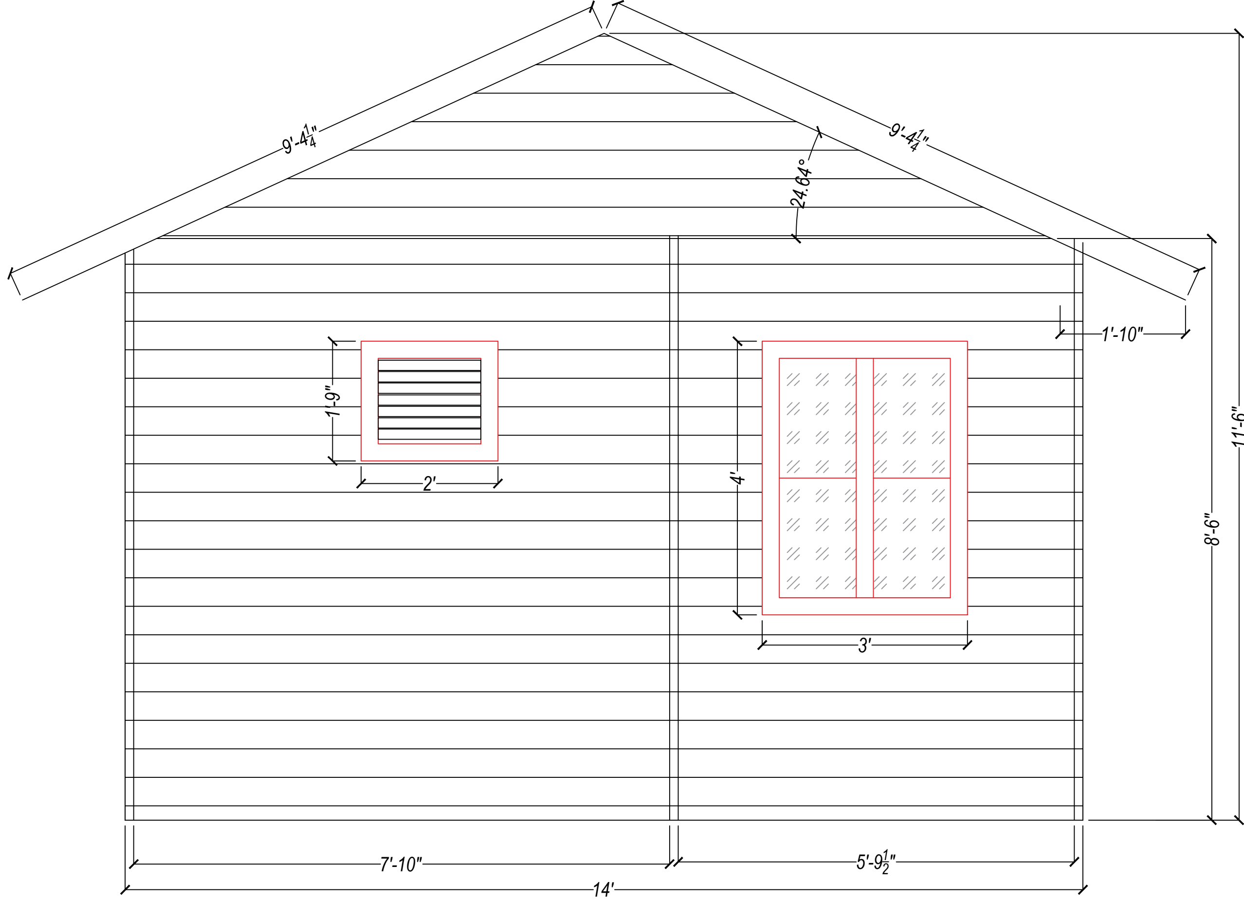
Back Elevation
