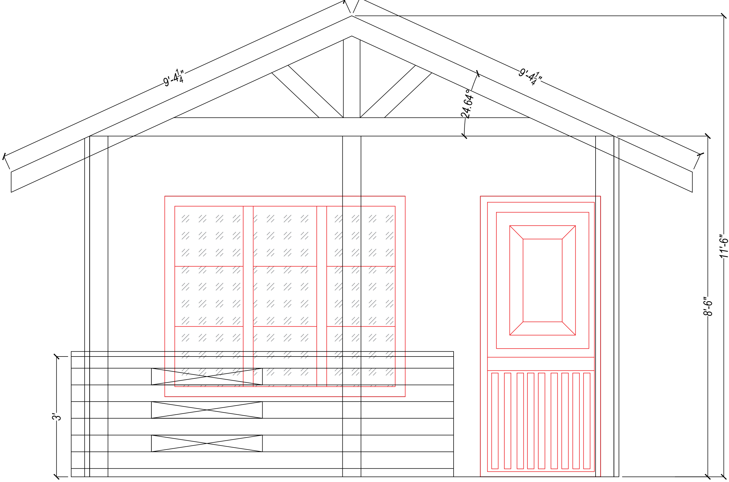
Left Elevation
